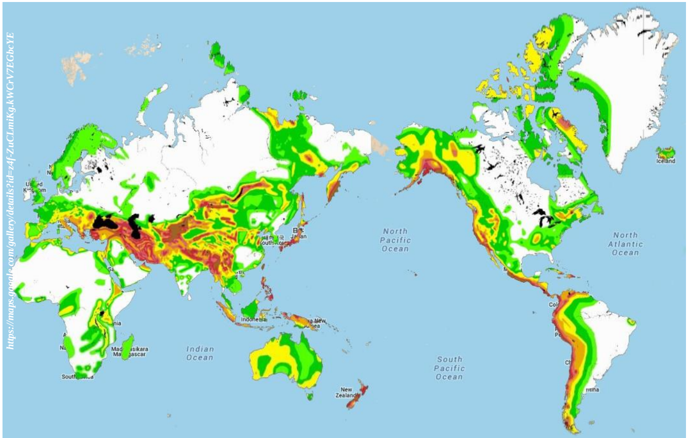
Global map of seismic hazard for 2014
